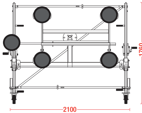
Technical Data (mm) Rotating Frame
